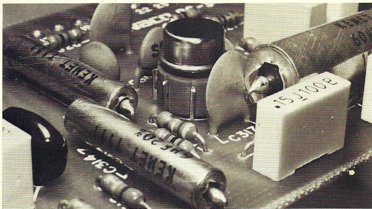
Mill-grade tantalum capacitors and FET-input Op Amp
